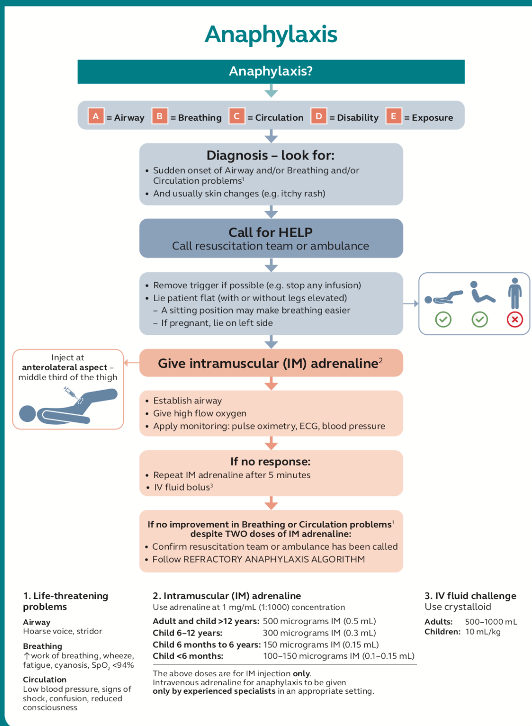
Figure 6. Anaphylaxis algorithm
